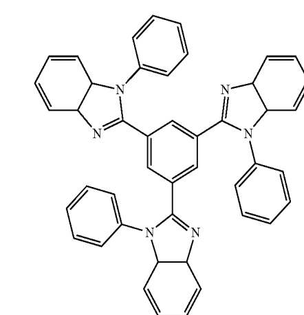
TPBI
