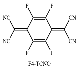
F4-TCNQ
